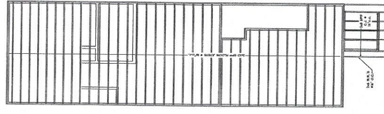
SECOND FLOOR FRAMING PLAN
