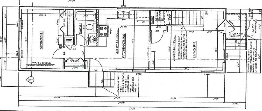
FIRST FLOOR PLAN HEATED AREA: 100 SQFT.
