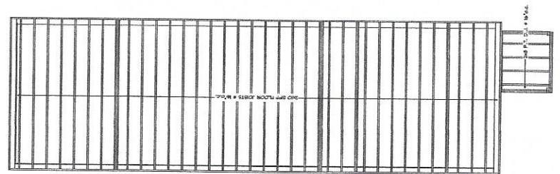
FIRST FLOOR FRAMING PLAN
