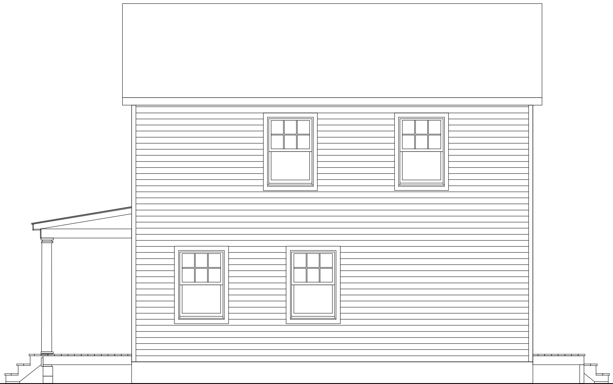
RIGHT SIDE YARD EXTERIOR ELEVATION SCALE: 1/4" = 1' - 0"
