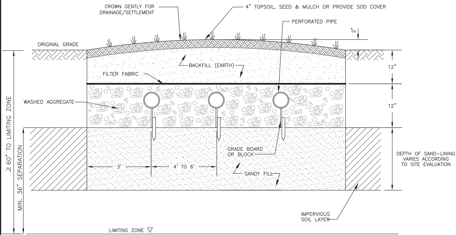
BED SECTION
