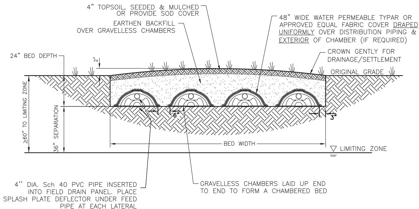
FULL DEPTH BED SECTION
