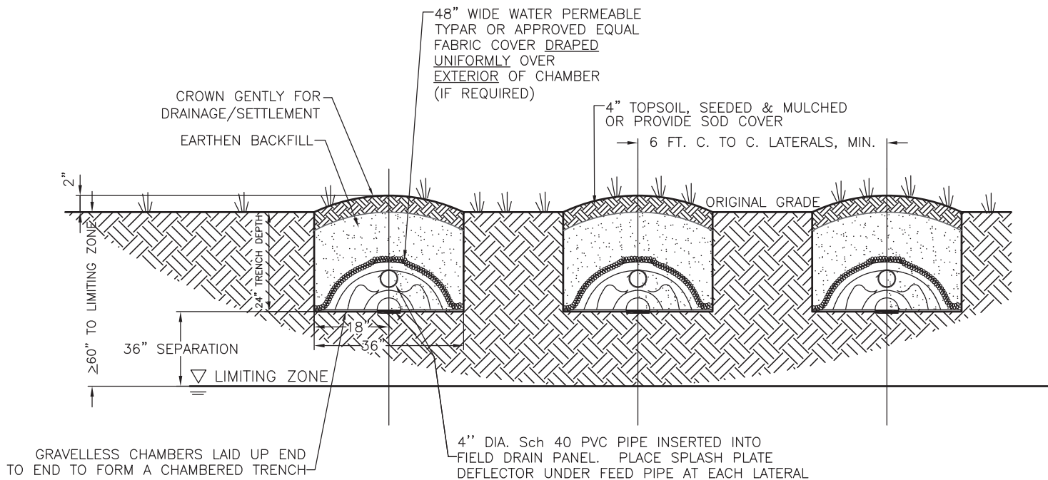
FULL DEPTH TRENCH SECTION
