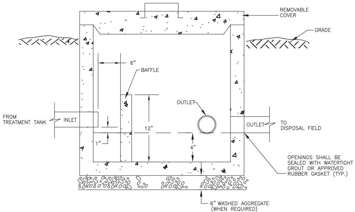
SECTION
