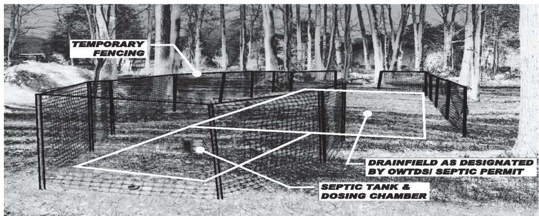
SAMPLES OF TEMPORARY BARRIERS/ BARRICADES FOR OWTDS
