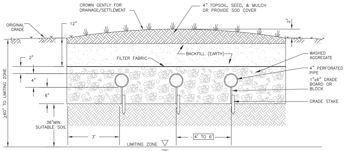
SECTION
