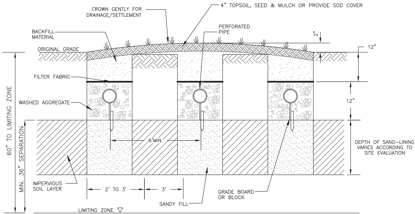
TRENCH SECTION
