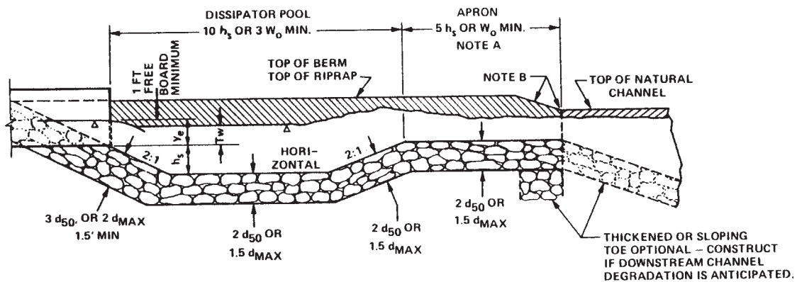
Profile thru Basin
