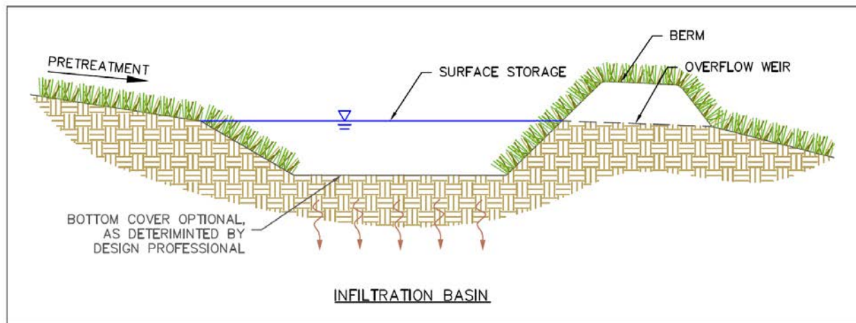
Figure 1.2 Infiltration Basin (Section View)
