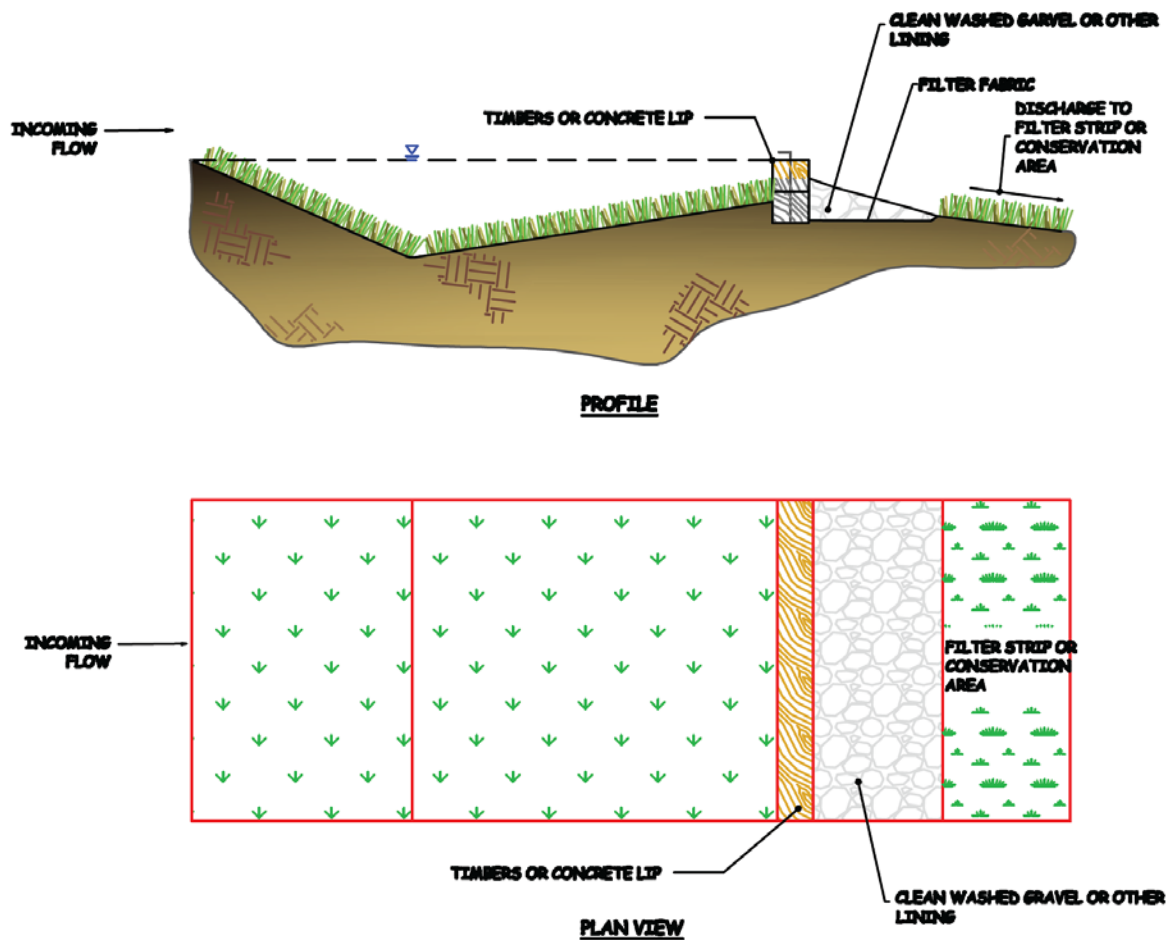
Figure 9.3: Example Level Spreader
