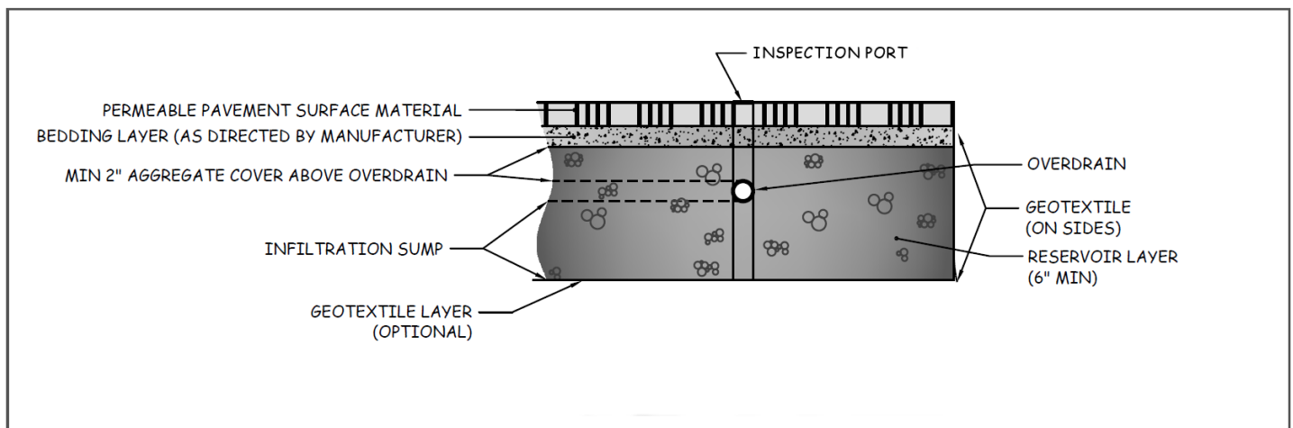
Figure 3.2 Permeable Pavement with Infiltration Sump and Overdrain
