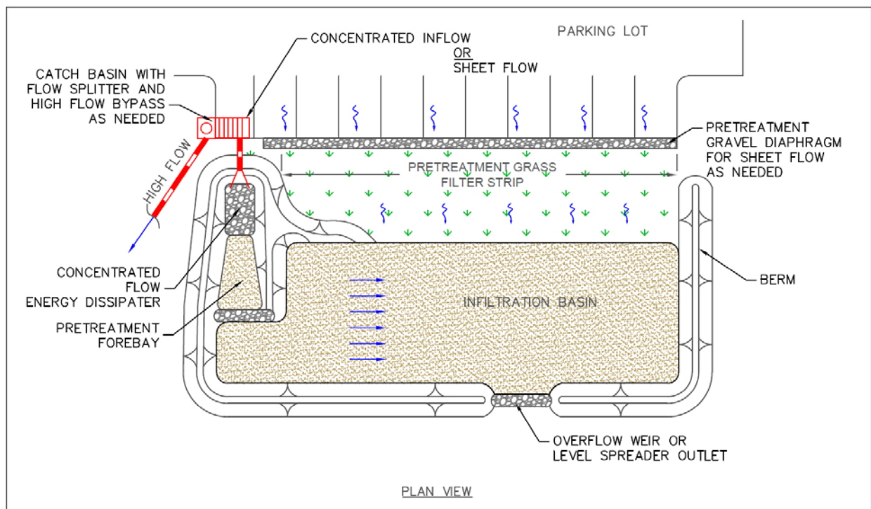
Figure 1.3 Infiltration Basin (Plan View)
