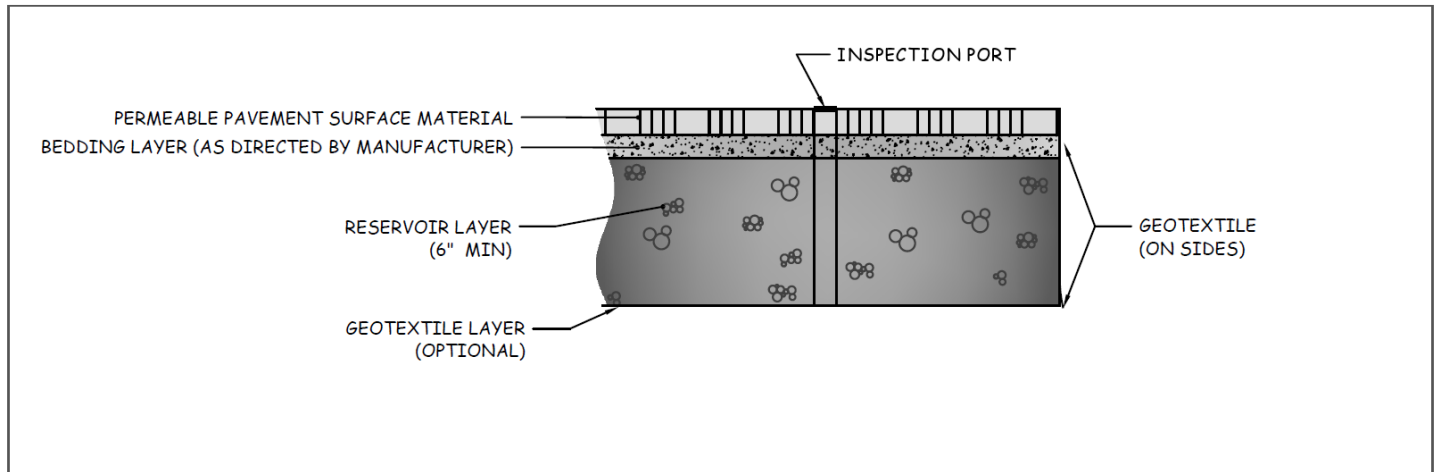
Figure 3.1 Permeable Pavement – Infiltrating
