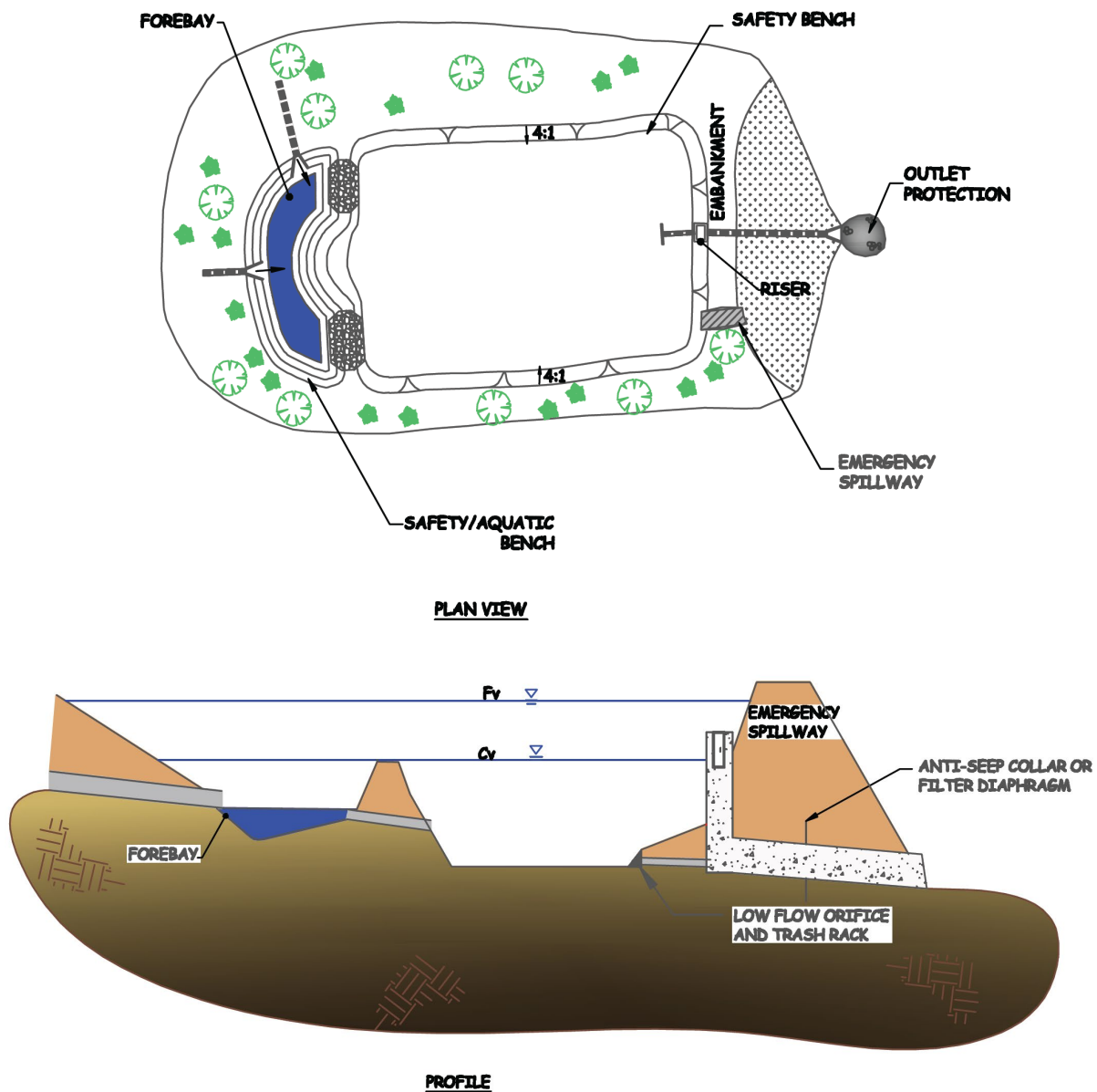
Figure 10.1. Example of a Dry Detention Pond (10-A)
