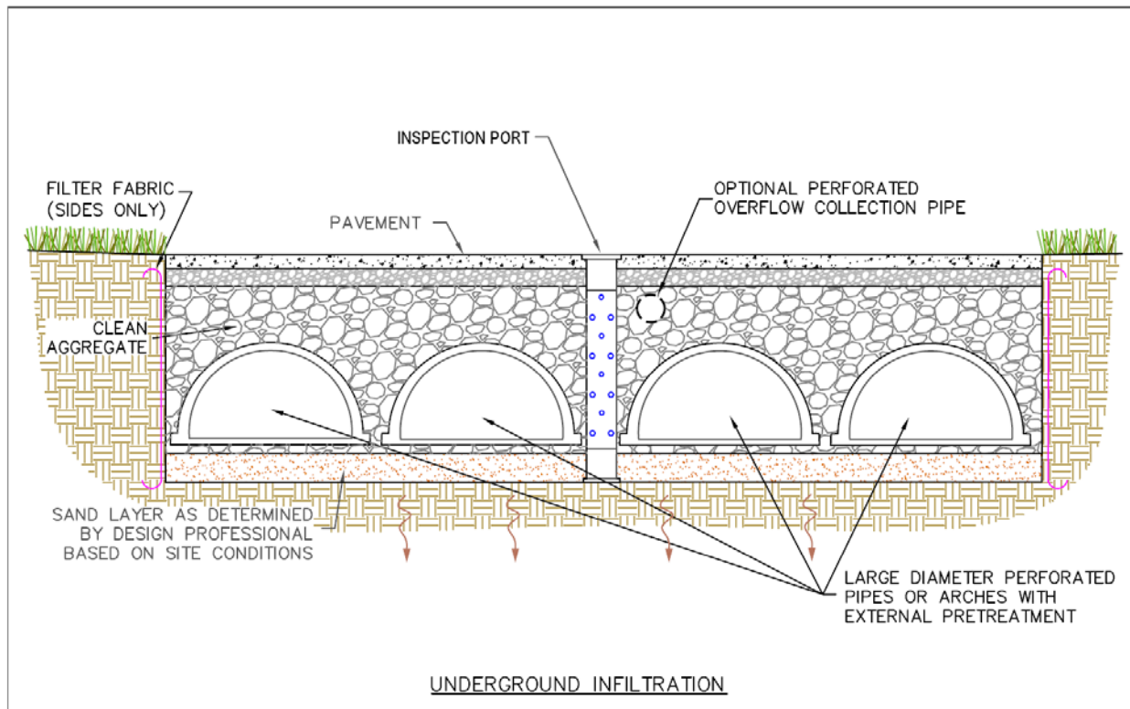
Figure 1.4 Underground Infiltration
