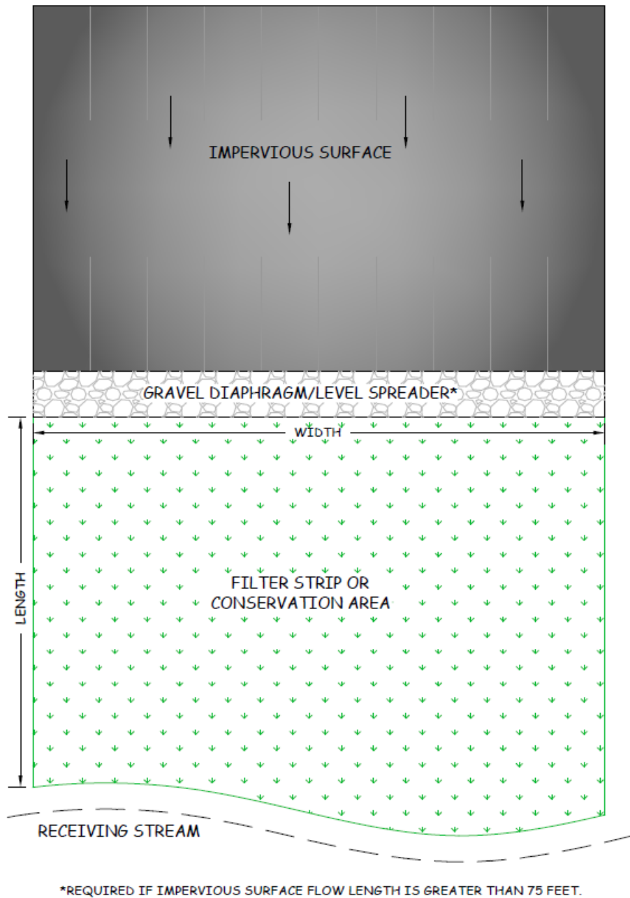
Figure 9.1. Sheet Flow to Vegetated Filter Strip or Vegetated Open Space
