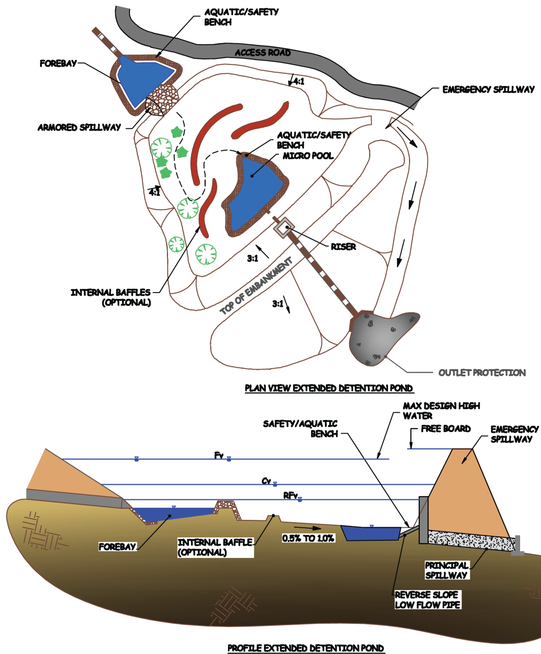
Figure 10.2. Example of a Dry Extended Detention Basin (10-B)
