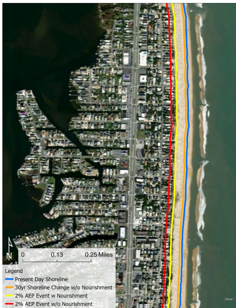
Figure 14-3. Current and future projected shoreline position, as well as shoreline position following a two percent AEP storm event with and without nourishment at Fenwick Island
