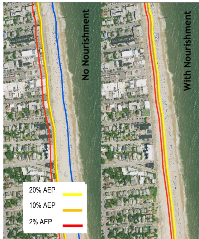
Figure 2-3. Example of episodic erosion modeling results showing the location of the eroded shoreline for storms of different magnitude along a section of Rehoboth Beach without (left) and with (right) nourishment.
