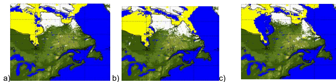
Figure 2. Snow depth and ice cover maps for northern Quebec from the last day of May in a) 2026, b) 2025, c) 2024 (Source: NOAA)
