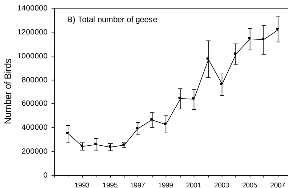
Fig. 3. Estimated number ( \pm 1 SE) of total Canada geese on the Ungava Peninsula, Québec, Canada, 1988 and 1993-2007.
